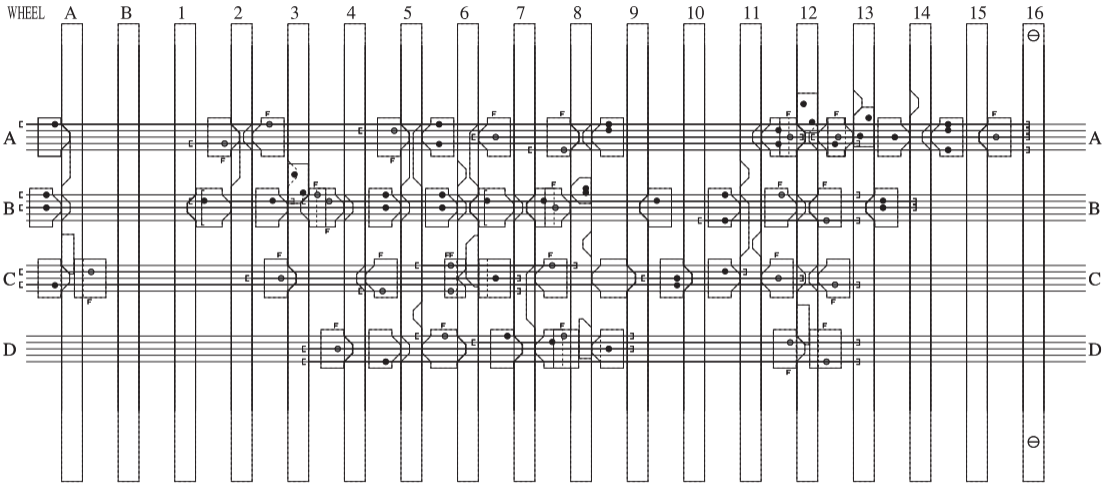
COLTHROP SIDING (PLAN) MECHANICAL LOCKING S 186/6
